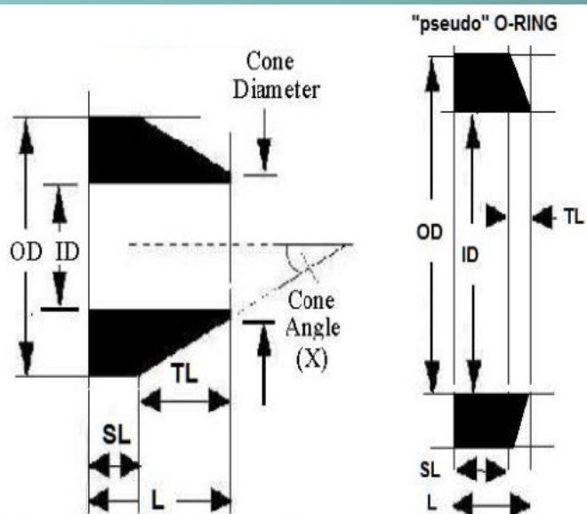
One-Piece Swagelok Cone Ferrule SF400G SF30.0/25.4/6.0-4.2-1.8G
