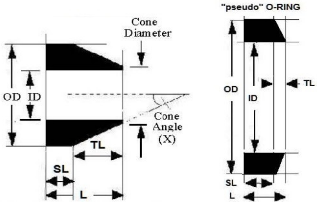
One-Piece Swagelok Cone Ferrule SF400G SF30.0/25.4/6.0-4.2-1.8G
