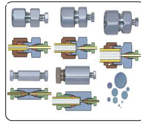
HPLC End-Fittings
