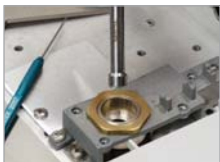
Slip tool over FID jet...
