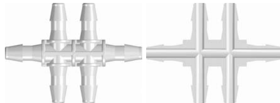
6PTT230 (-1 -6) Six-port Thru Flow Double T Style Manifold with 200 Series Barbs for 1/8" (3.2 mm) ID Tubing
