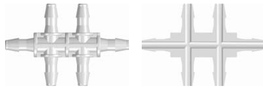
6PTT230 (-1 -6) Six-port Thru Flow Double T Style Manifold with 200 Series Barbs for 1/8" (3.2 mm) ID Tubing
