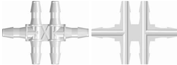
6PTT210 (-1 -6) Six-port Thru Flow Double T Style Manifold with 200 Series Barbs for 1/16" (1.6 mm) ID Tubing
